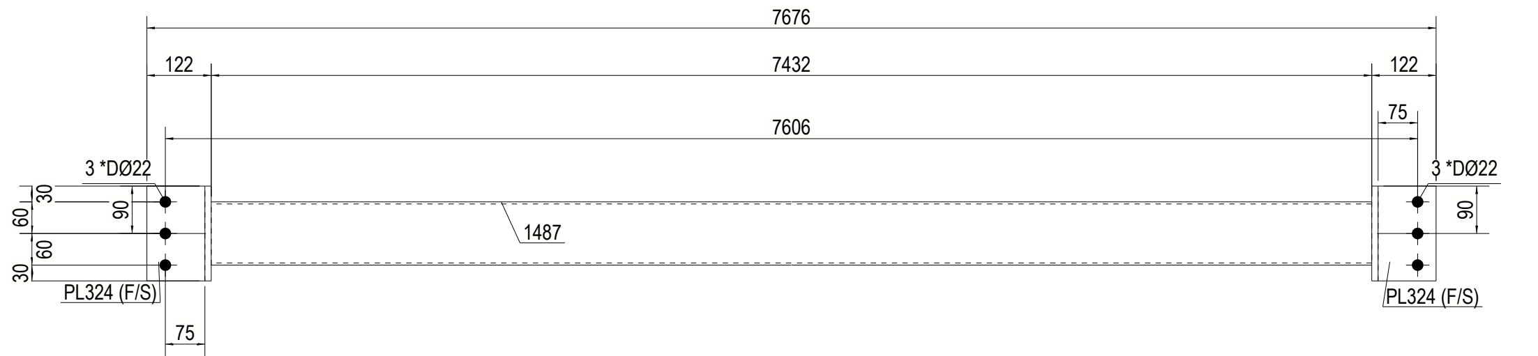
FRONT VIEW
